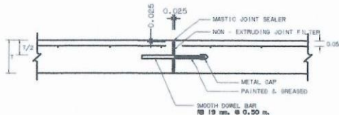
EXPANSION JOINT
