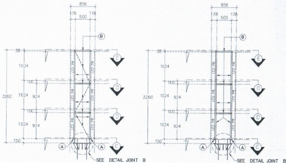
SECTION A TRUSS (T1-T5) SCALE 1 : 50
